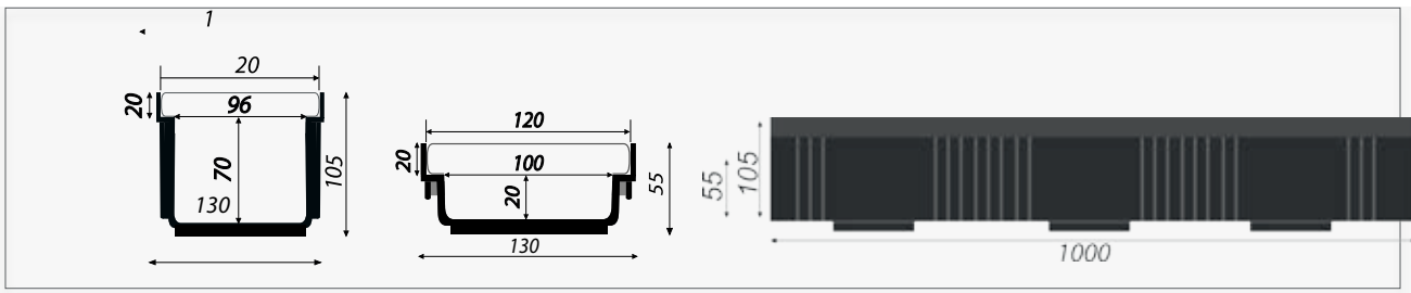
Technical sections of linear drain
